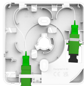
FiberTwist Bracket-2-patch-in
