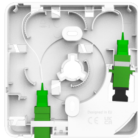
FiberTwist Bracket-2-patch-in
