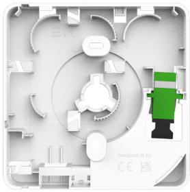
FiberTwist Bracket-2
